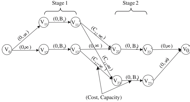
Fig. 1. Network flow model of Case II of the FFA problem
